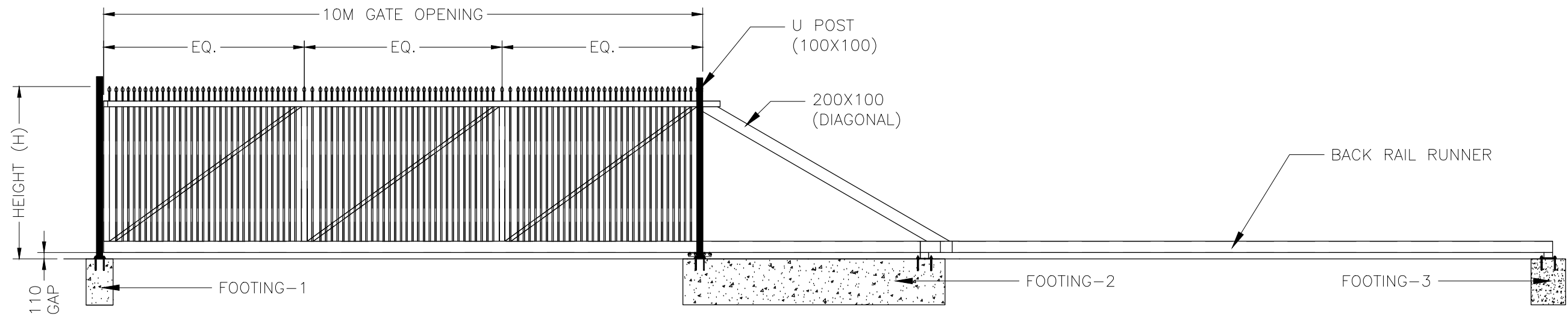
FRONT VIEW
