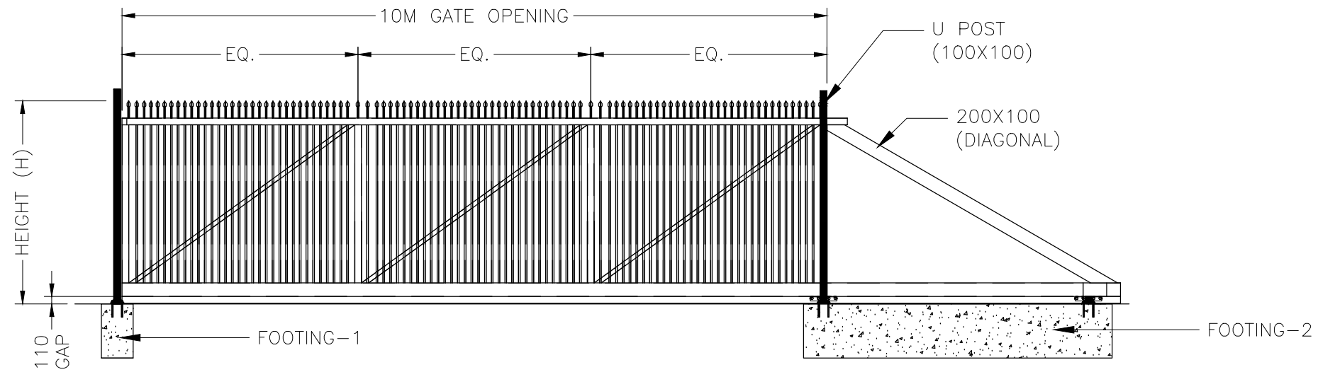
FRONT VIEW
