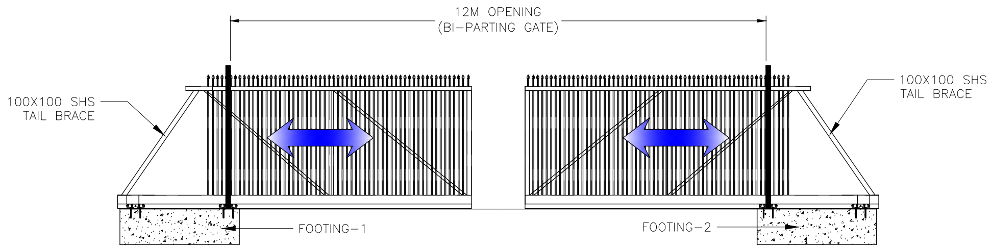
FRONT VIEW
