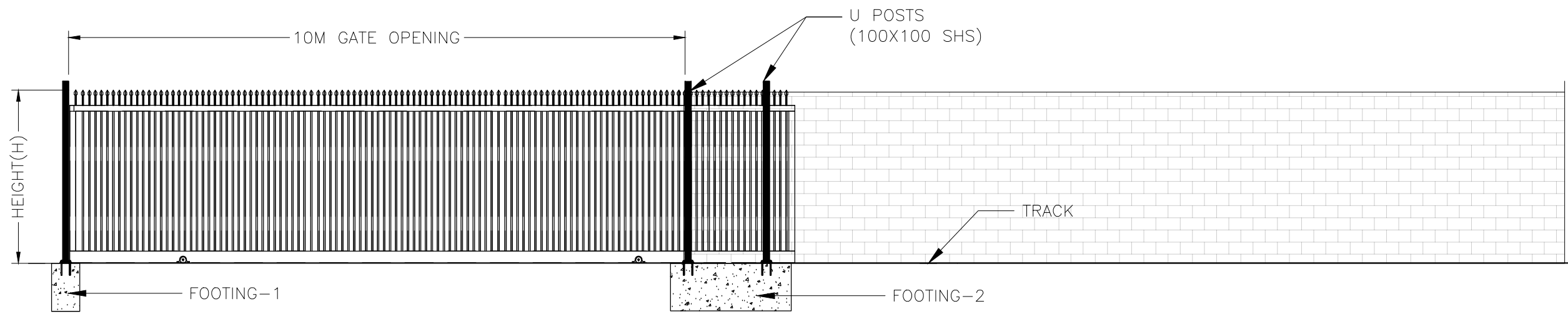
FRONT VIEW
